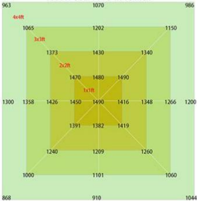
1000W 8bar PPFD in 18 inch
