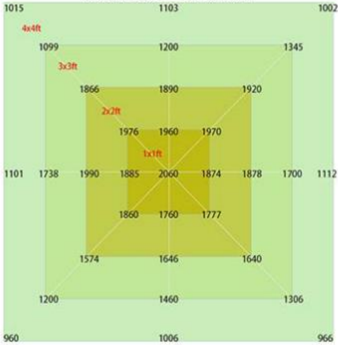
1000W 8bar PPFD in 6 inch
