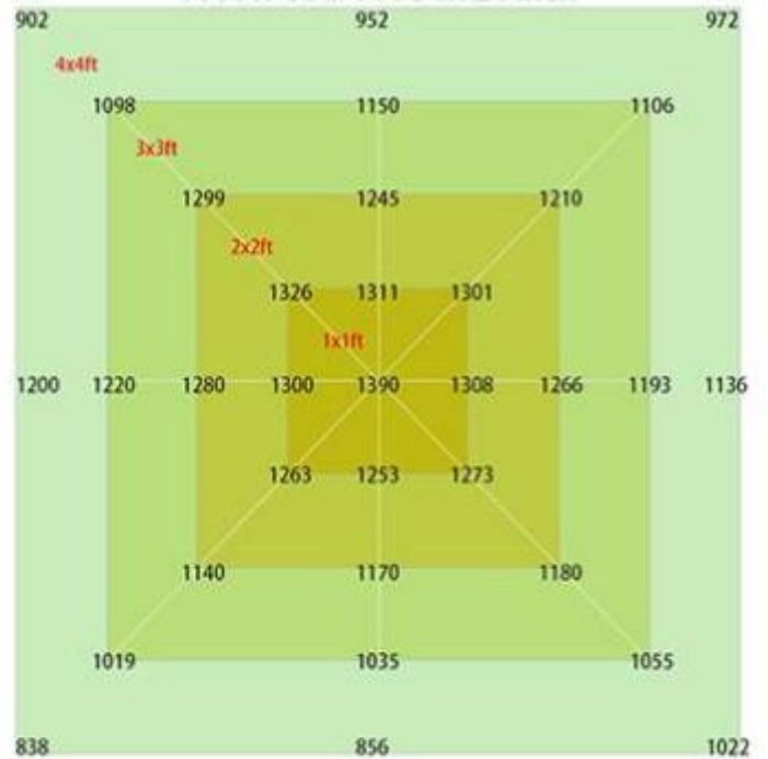
1000W 8bar PPFD in 24 inch
