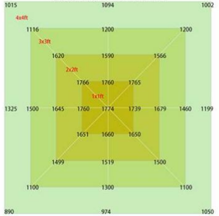
1000W 8bar PPFD in 12 inch
